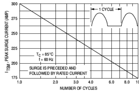
Maximum Non-Repetitive Surge Current
