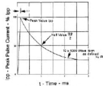
FIGURE 2 Test waveform parameters: t_r=10 \mu s , t_p=1000 \mu s Pulse Waveform
