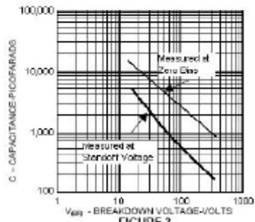
FIGURE 3 Typical Capacitance vs. Breakdown Voltage
